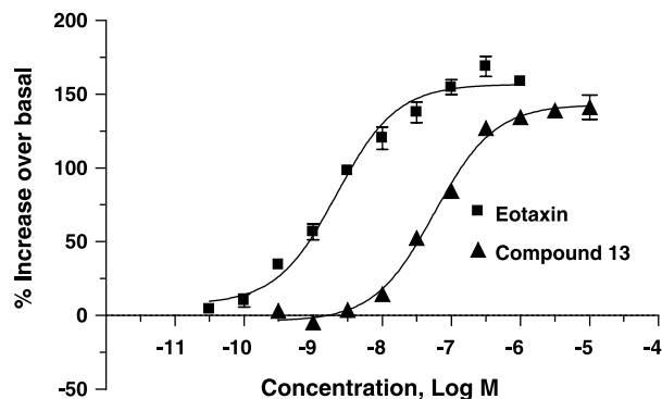
Figure 1. CCR3 35 S-GTP \gamma S binding for eotaxin and compound 13 .
