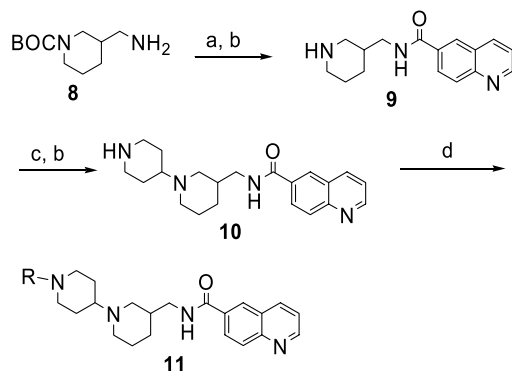
Scheme 2. Reagents and conditions: (a) 6-quinolinecarboxylic acid, EDCI, HOBT, \text{CH}_2\text{Cl}_2 , 96%; (b) TFA, \text{CH}_2\text{Cl}_2 , 100%; (c) N -BOC-4-piperidone, AcOH, \text{NaB}(\text{OAc})_3\text{H} , \text{CH}_2\text{Cl}_2 , 70%; (d) \text{RCHO} , AcOH, \text{NaB}(\text{OAc})_3\text{H} , \text{CH}_2\text{Cl}_2 or \text{RCOCl} , \text{Et}_3\text{N} , \text{CH}_2\text{Cl}_2 .
