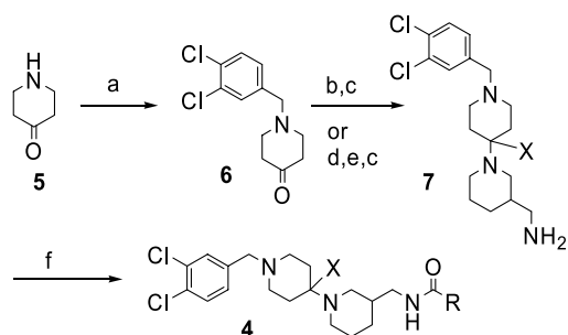
Scheme 1. Reagents and conditions: (a) 3,4-dichlorobenzyl chloride, \text{Et}_3\text{N} , \text{ClCH}_2\text{CH}_2\text{Cl} , \Delta , 65%; (b) 3-( t BOC-aminomethyl)piperidine, \text{CH}_2\text{Cl}_2 , \text{AcOH} , \text{NaB}(\text{OAc})_3\text{H} , 64% for \text{X} = \text{H} ; (c) \text{TFA} , \text{CH}_2\text{Cl}_2 , 100%; (d) 3-( t BOC-aminomethyl)-piperidine, \text{Ti}(\text{OiPr})_4 , \text{CH}_2\text{Cl}_2 , \text{Et}_2\text{AlCl} , 96% for \text{X} = \text{CN} ; (e) \text{MeMgBr} , \text{THF} , 0^\circ\text{C} , 88% for \text{X} = \text{Me} ; (f) \text{RCOOH} , \text{Et}_3\text{N} , \text{EDCI} , \text{HOBT} , \text{DMF} .
